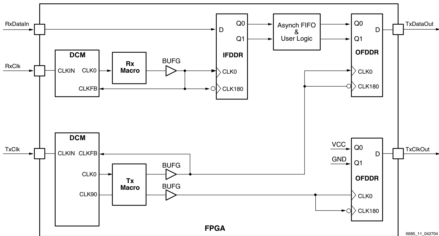
Figure 5: Design with Local Inversion Clock Macro
