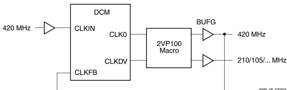
Figure 11: Corner 2VP100 DCM Example Circuit 3
