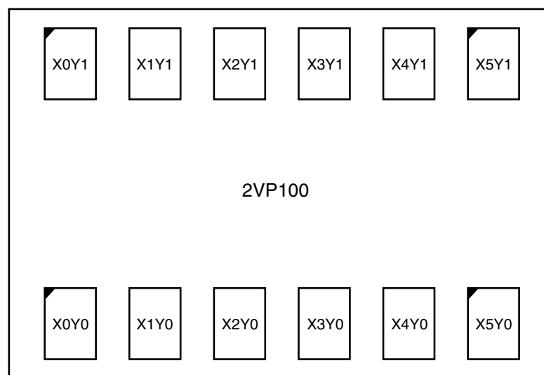
Figure 8: 2VP100 with Corner DCMs
