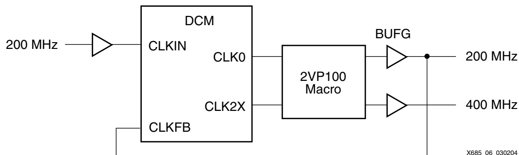
Figure 9: Corner 2VP100 DCM Example Circuit 1
