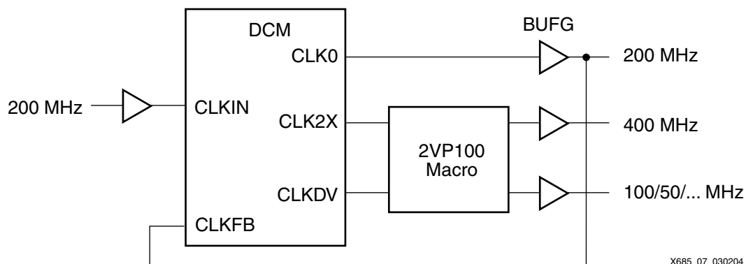
Figure 9: Corner 2VP100 DCM Example Circuit 1
